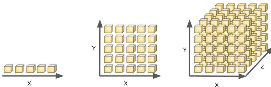
Figure 8: An illustration of the curse of dimensionality
