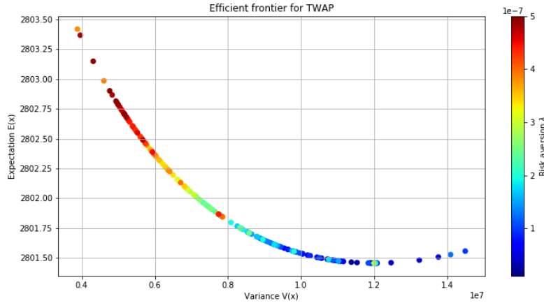
Figure 6: Efficient frontier for TWAP
